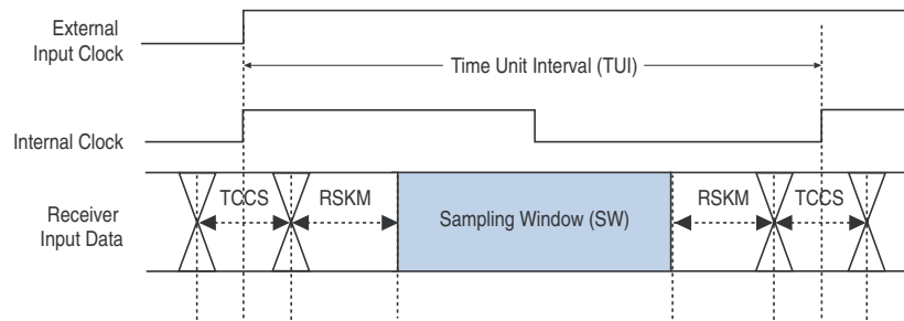
Figure 8–25. High-Speed I/O Timing Diagram
