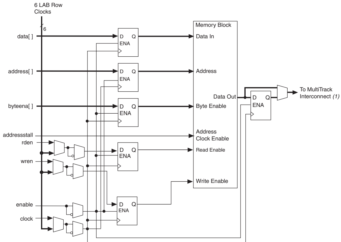
Figure 4–21. Cyclone III Single-Clock Mode in Single-Port Mode
