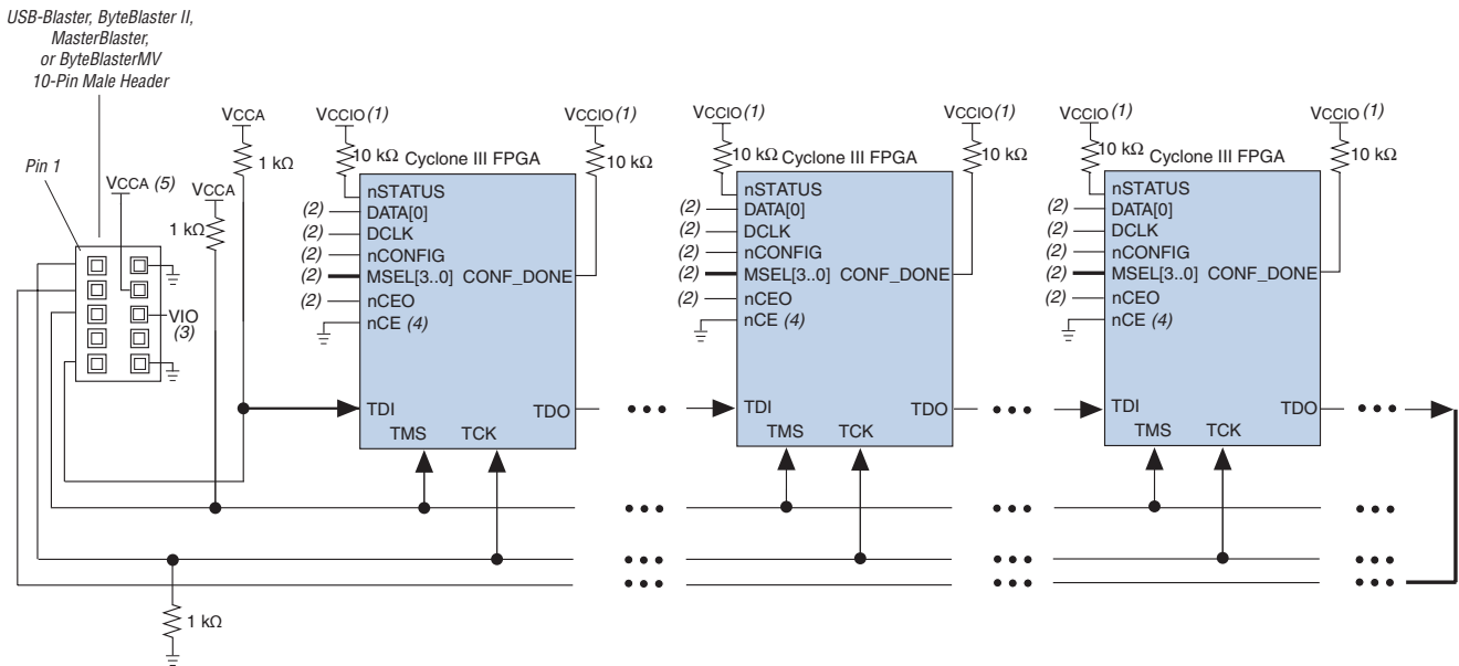
Figure 10–26. JTAG Configuration of Multiple Devices Using a Download Cable (2.5 V, 3.0 V, or 3.3 V V_{CCIO} Powering the JTAG Pins)
