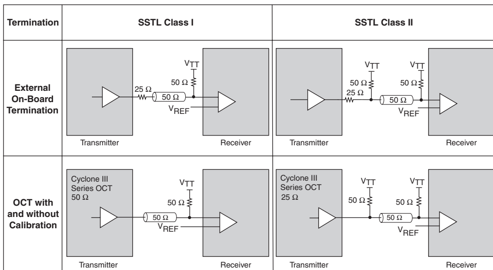
Figure 7–12. Cyclone III SSTL I/O Standard Termination
