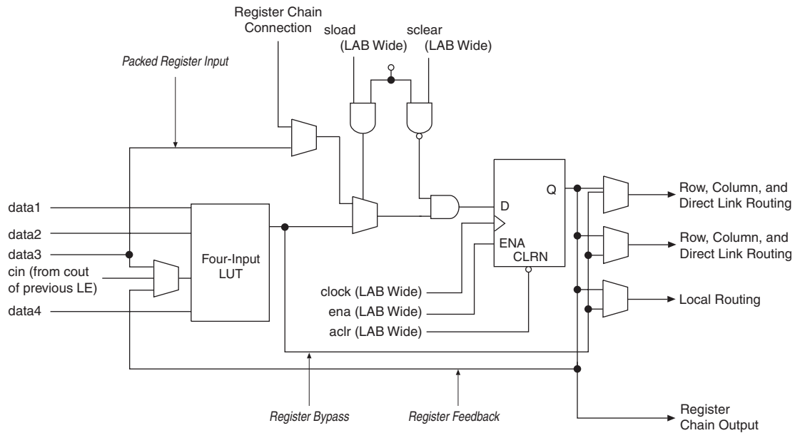
Figure 2-4. LE in Normal Mode
