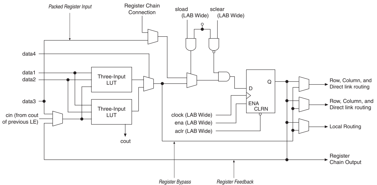
Figure 2-5. LE in Arithmetic Mode
