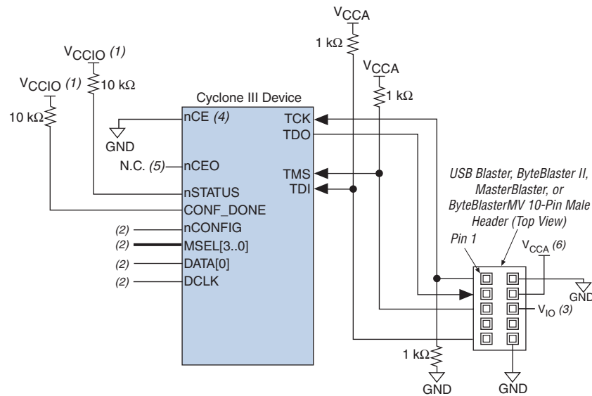
Figure 10–24. JTAG Configuration of a Single Device Using a Download Cable (2.5 V, 3.0 V, or 3.3 V V_{CCIO} Powering the JTAG Pins)
