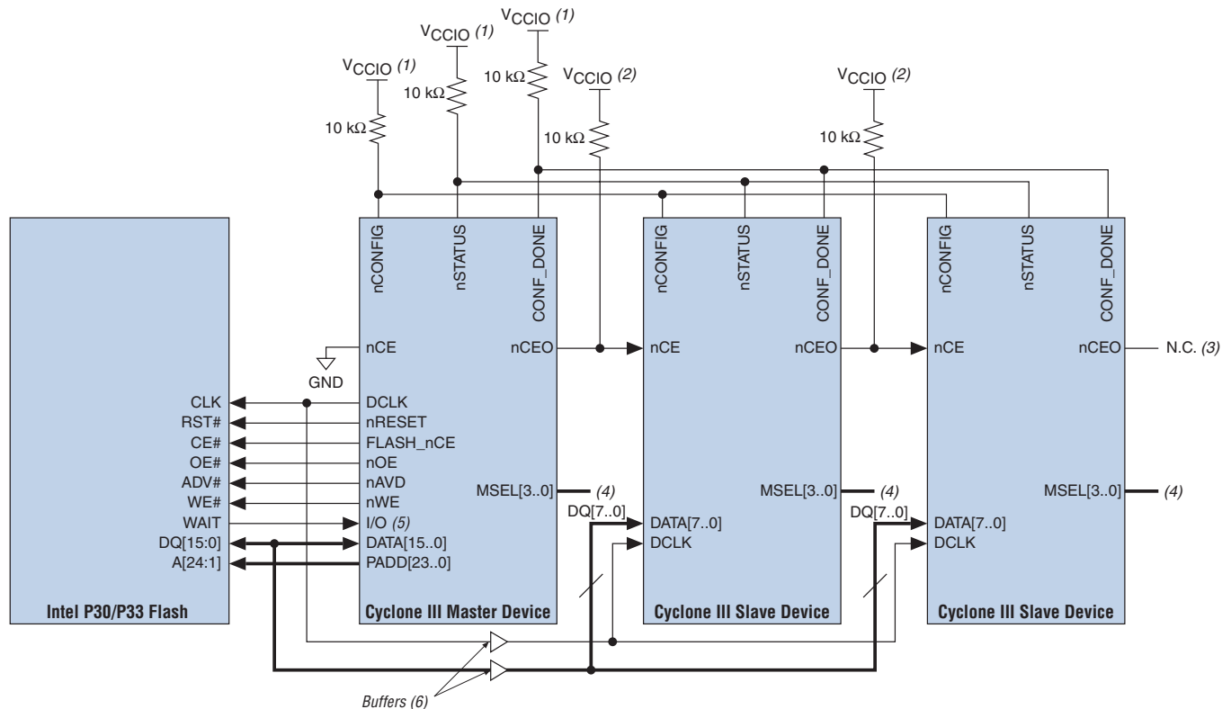
Figure 10–9. Byte-Wide Multi-Device AP Configuration
