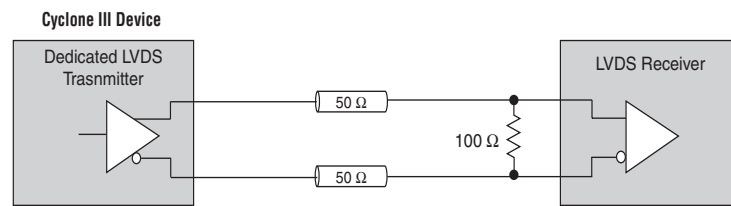
Figure 8–3. LVDS Interface with Dedicated Output Buffer on the Left and Right I/O Banks
