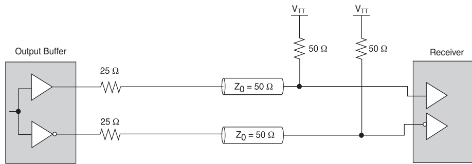
Figure 8–20. Differential SSTL Class I Interface
