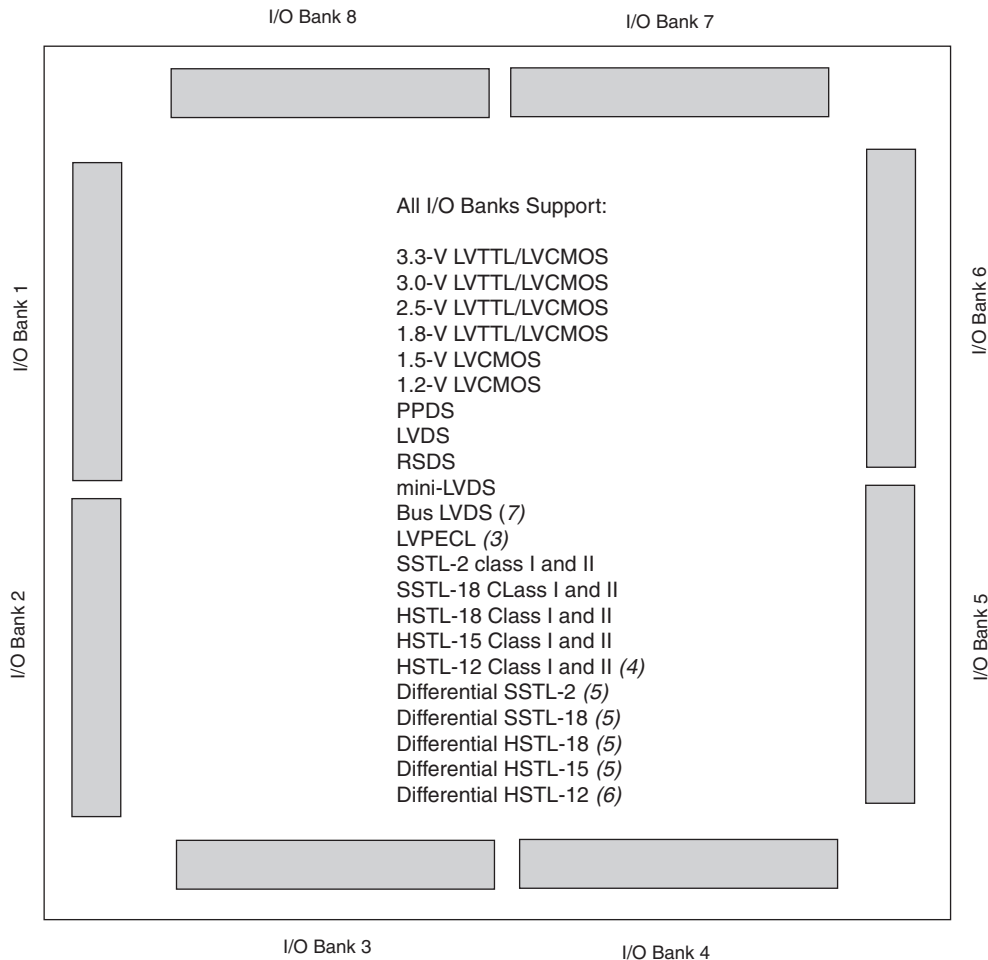
Figure 7–15. Cyclone III Device I/O Banks Notes (1), (2)
