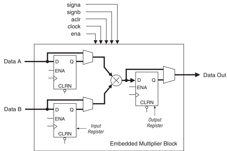
Figure 5–2. Multiplier Block Architecture
