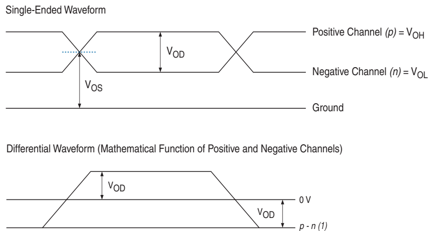
Figure 8–15. Transmitter Output Signal Level Waveforms for PPDS
