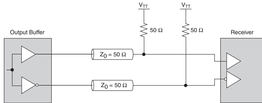
Figure 8–22. Differential HSTL Class I Interface
