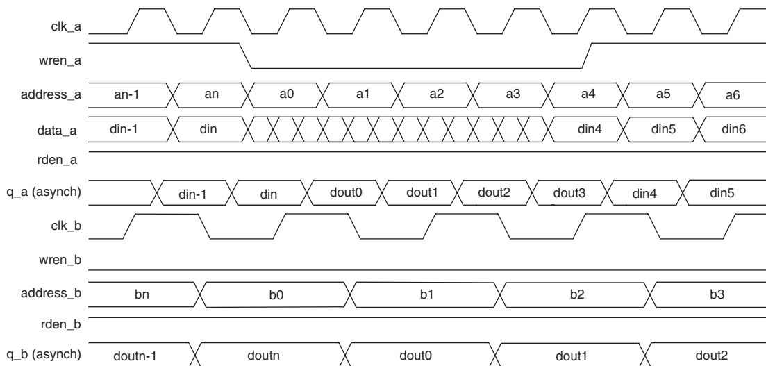
Figure 4-12. Cyclone III True Dual-Port Timing Waveforms
