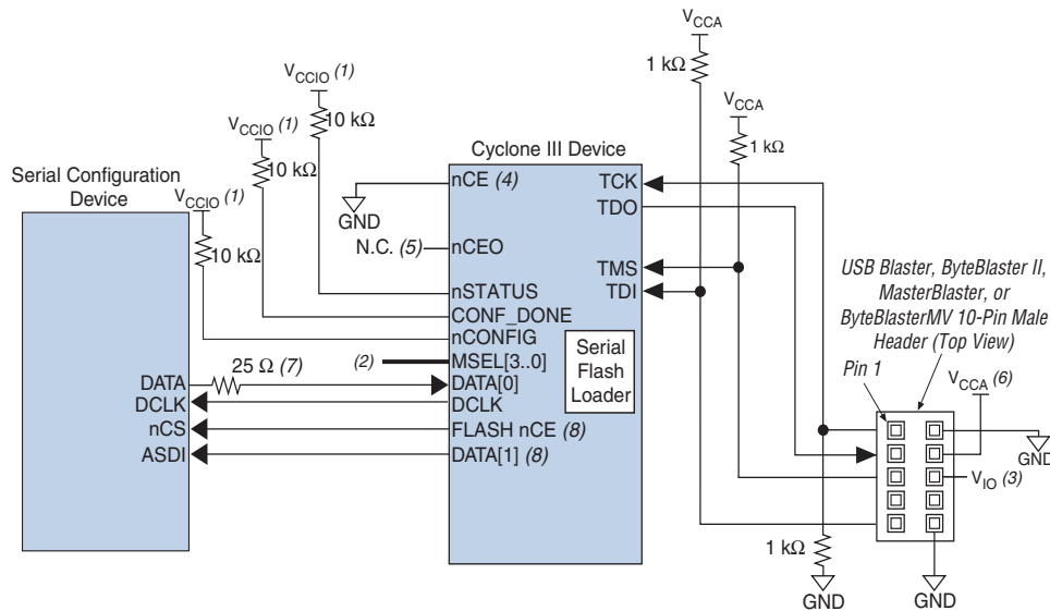
Figure 10–30. Programming Serial Configuration Devices In-System Using the JTAG Interface
