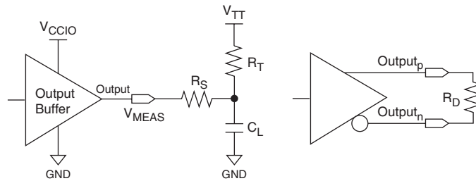
Figure 1–4. Output Delay Timing Reporting Setup Modeled by Quartus II Software for Single-Ended Outputs and Dedicated Differential Outputs Notes (1), (2)
