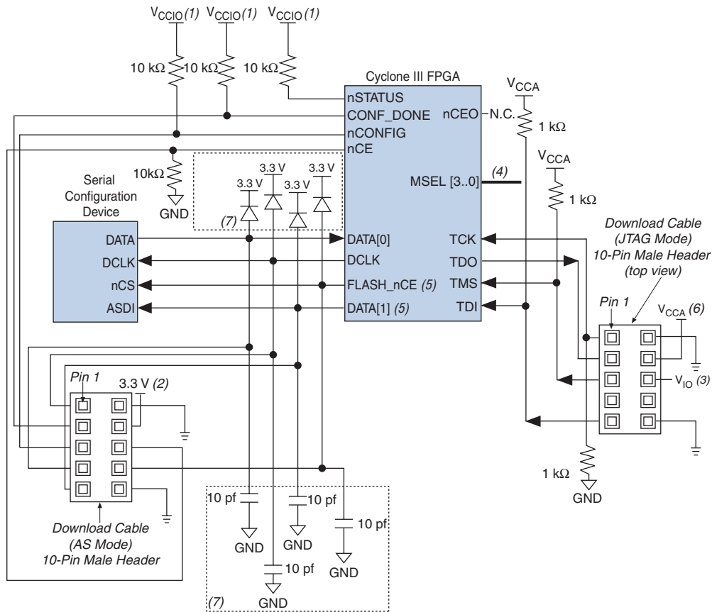
Figure 10–29. Combining JTAG and AS Configuration Schemes
