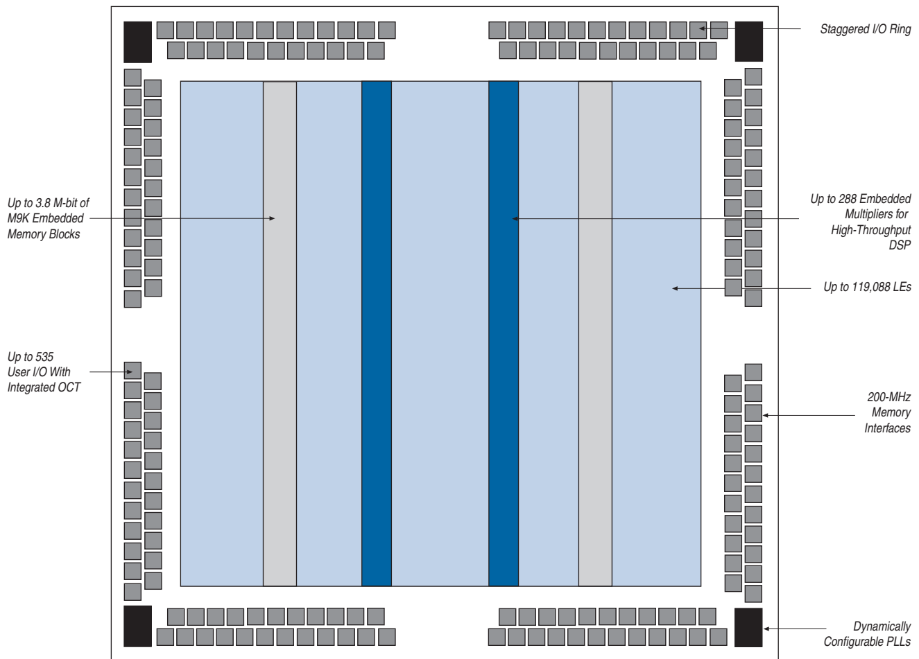
Figure 1–1. Cyclone III Device Architecture Overview Note (1)
