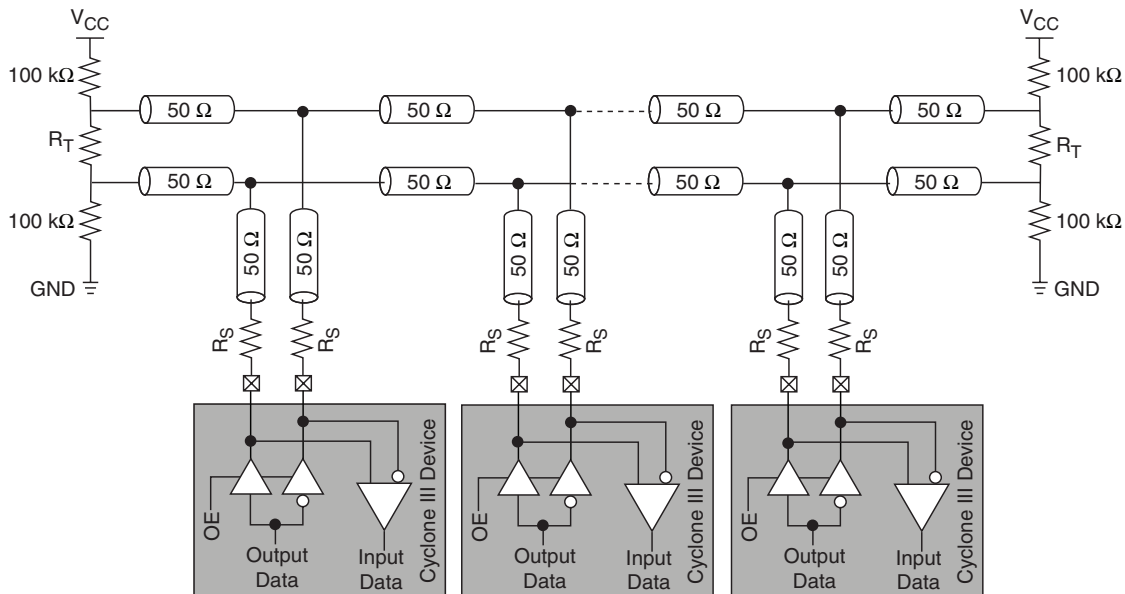
Figure 8–7. BLVDS Topology with Cyclone III Transmitters and Receivers
