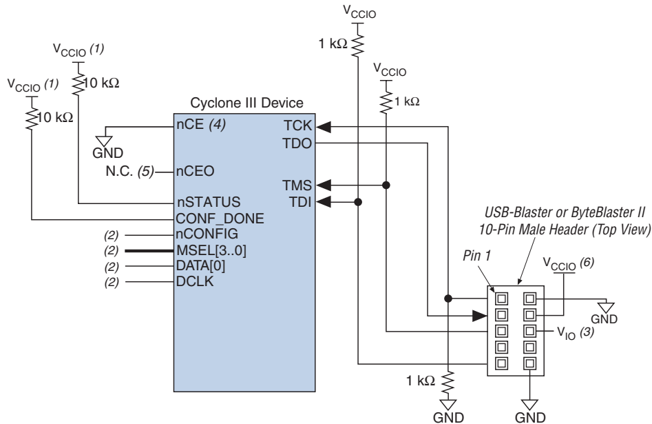
Figure 10–25. JTAG Configuration of a Single Device Using a Download Cable (1.5 V or 1.8 V V_{CCIO} Powering the JTAG Pins)
