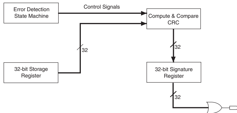
Figure 13-1. Error Detection Block Diagram
