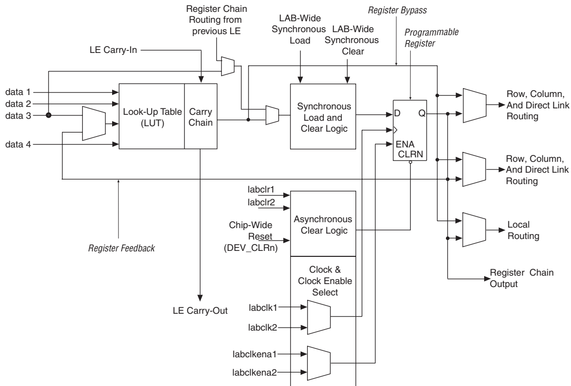
Figure 2–1. Cyclone III LE
