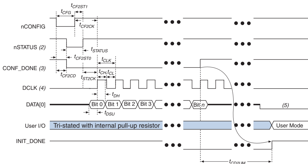
Figure 10–17. PS Configuration Timing Waveform Note (1)
