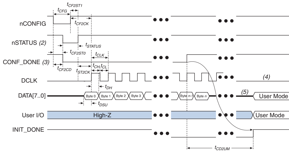
Figure 10–23. FPP Configuration Timing Waveform Note (1)
