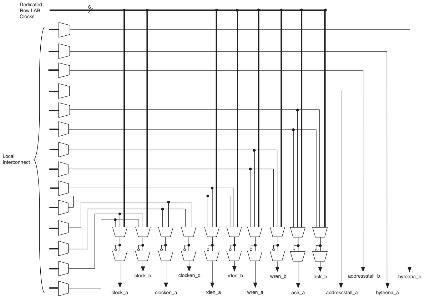
Figure 4–1. M9K Control Signal Selection
