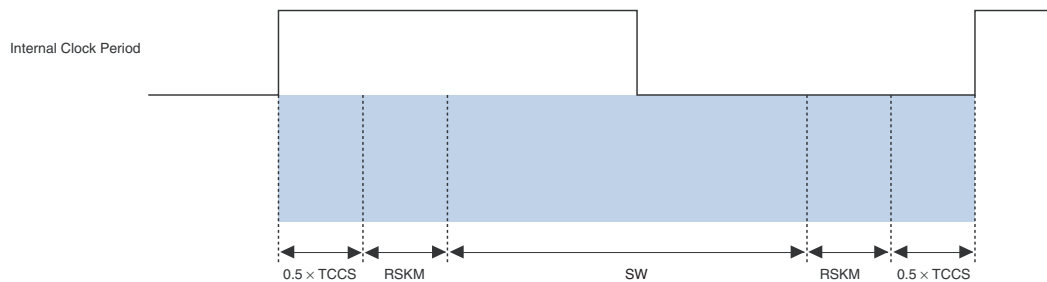
Figure 8–26. Cyclone III High-Speed I/O Timing Budget Note (1)
