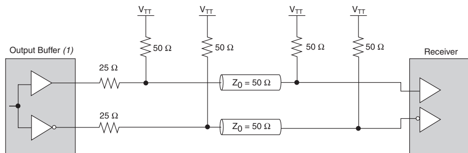
Figure 8–21. Differential SSTL Class II Interface
