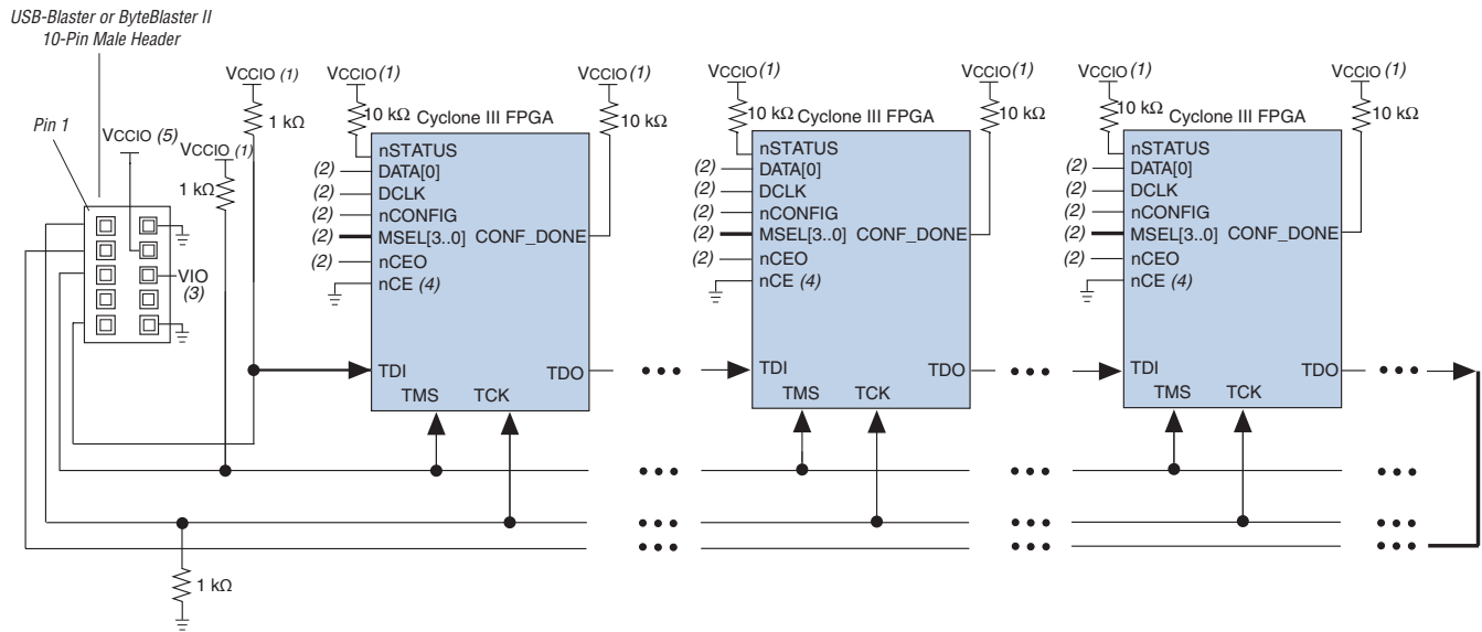
Figure 10–27. JTAG Configuration of Multiple Devices Using a Download Cable (1.2 V, 1.5 V, or 1.8 V V_{CCIO} Powering the JTAG Pins)
