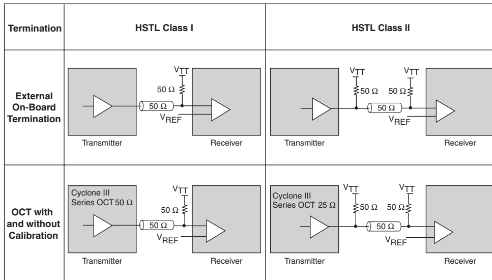
Figure 7–11. Cyclone III HSTL I/O Standard Termination
