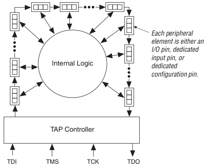
Figure 14–3. Boundary-Scan Register
