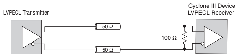
Figure 8–19. LVPECL DC-Coupled Termination
