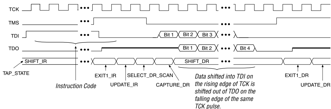
Figure 14–12. BYPASS Shift Data Register Waveforms
