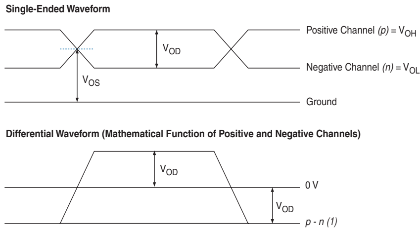
Figure 8–8. Transmitter Output Signal Level Waveforms for RSDS
