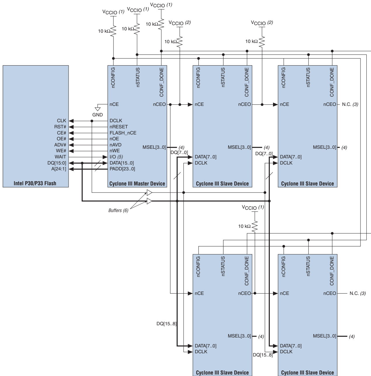
Figure 10–10. Word-Wide Multi-Device AP Configuration
