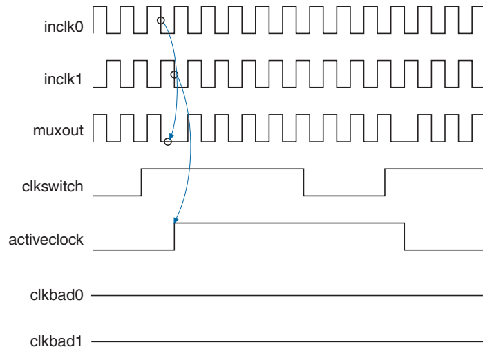
Figure 6–19. Clock Switchover Using the clkswitch Control
