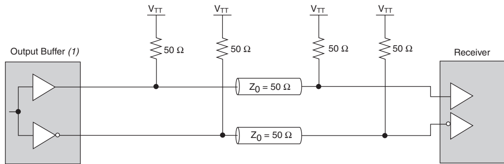
Figure 8–23. Differential HSTL Class II Interface
