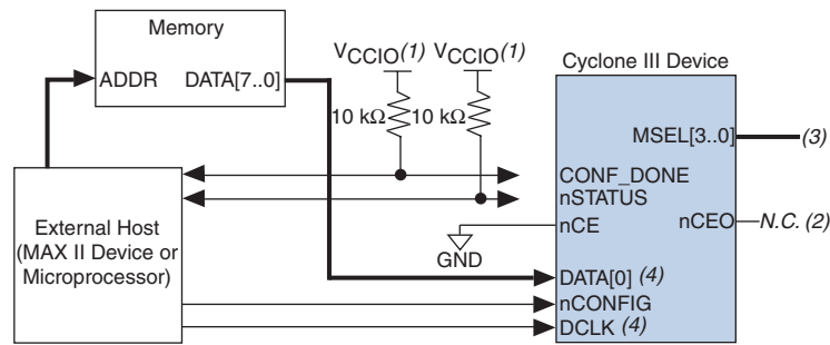
Figure 10–20. Single Device FPP Configuration Using an External Host
